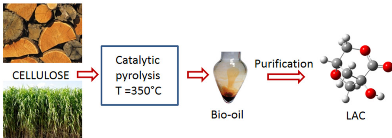
Fig. 1. Production of the anhydro-sugar LAC from cellulose pyrolysis
