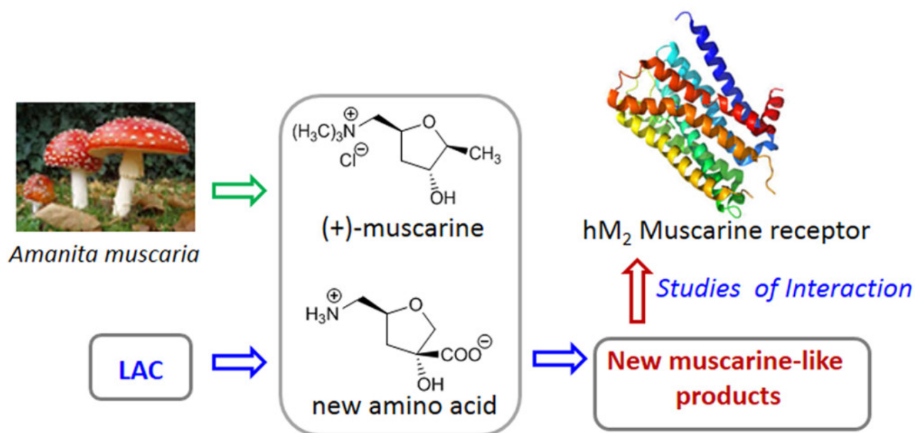
Fig. 2. Synthesis and biological evaluation of new the muscarine-like compounds synthesized from LAC via a new amino acid
